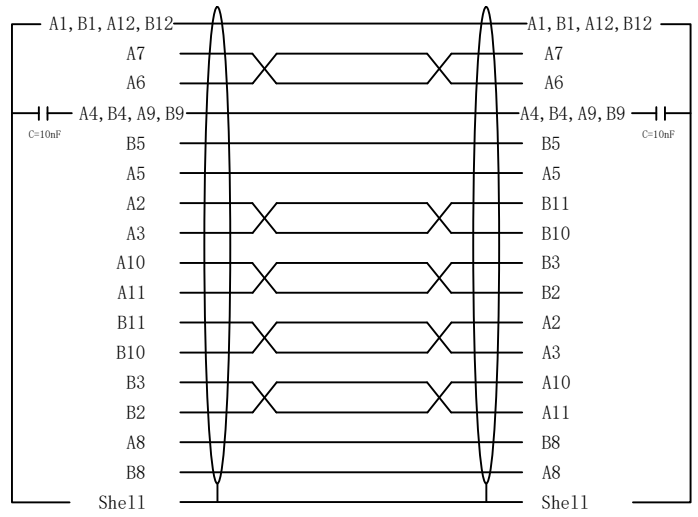
PIN OUT
