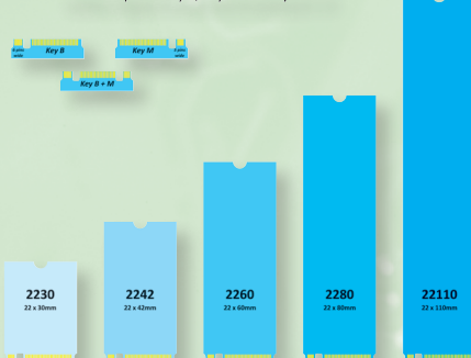
Contact Shapes of Key B, Key M and Key B + M
